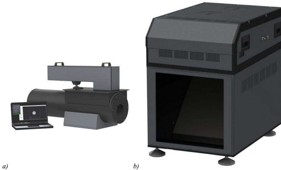
Fig. 2. Main blocks of LAFELD system: a) CIR imaging radiometer, b) RRT reference target
