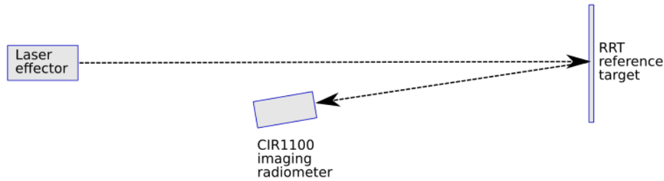
Fig. 1. Block diagram of LAFELD system
